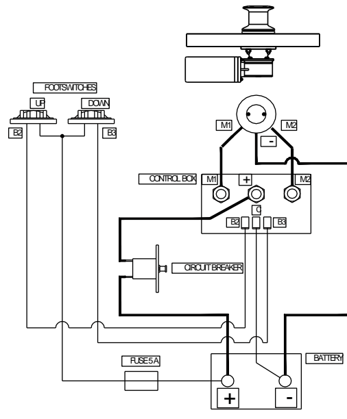
3 Terminals Motors
