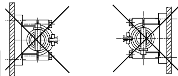
MONTAGE NON CONFORME / WRONG MOUNTING
