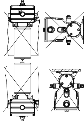
MONTAGE NON CONFORME WRONG MOUNTING
